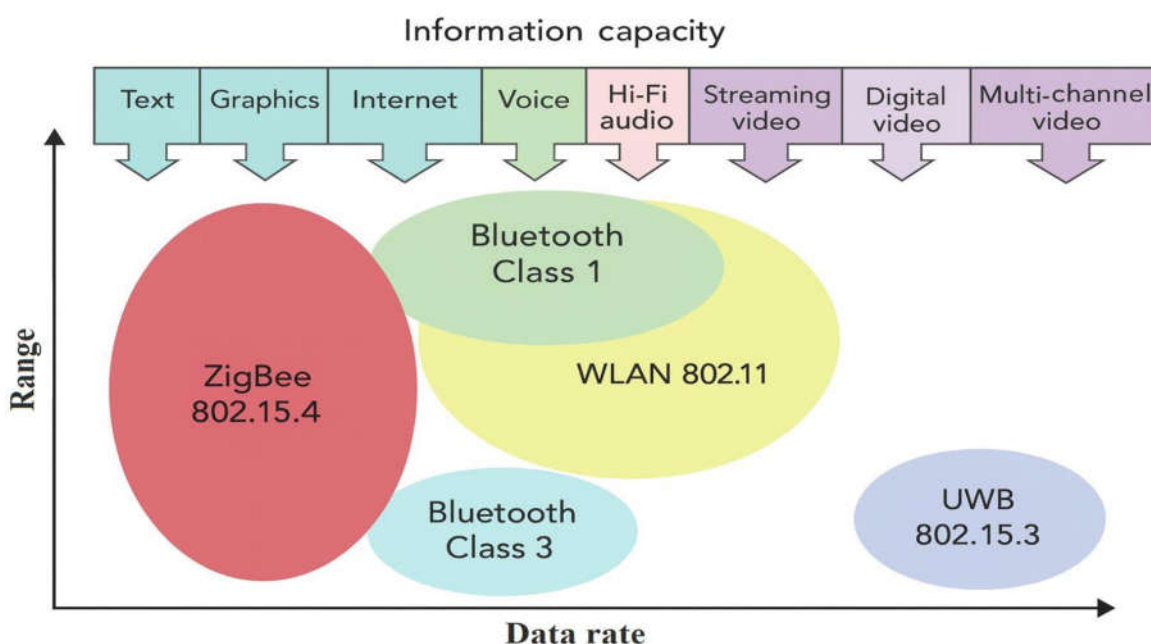
Figure 1 – Classification of some wireless standards
